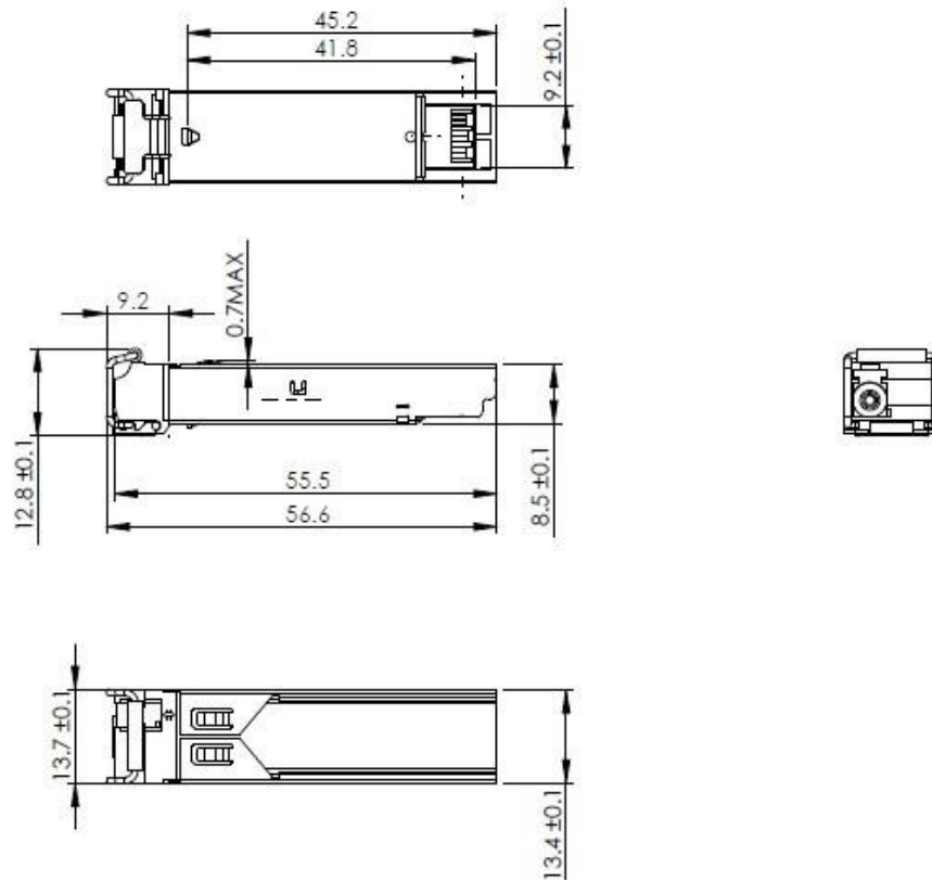
Mechanical Drawing
