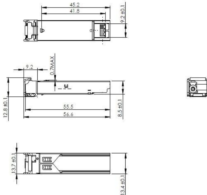
Mechanical Drawing
