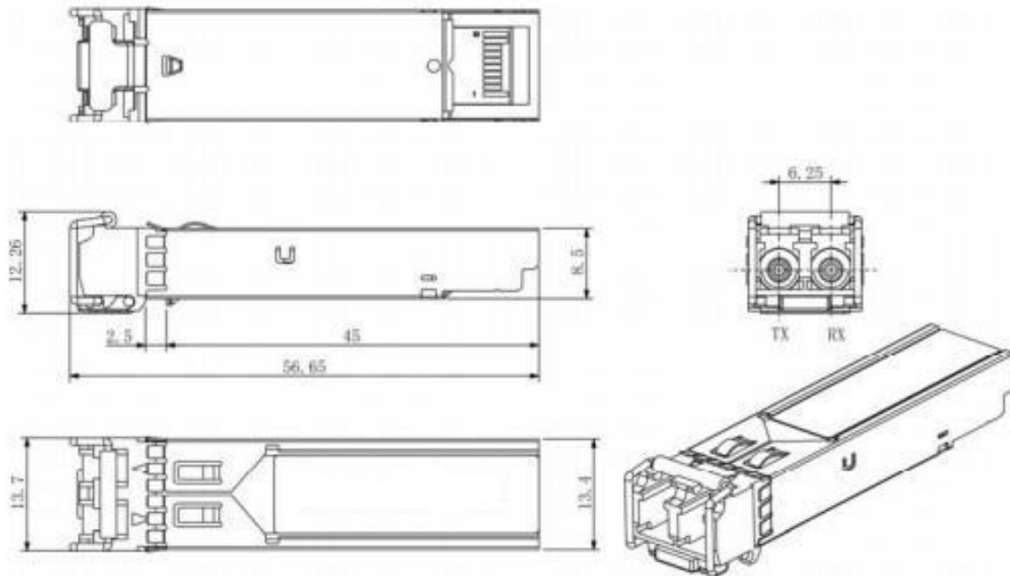
Mechanical Drawing
