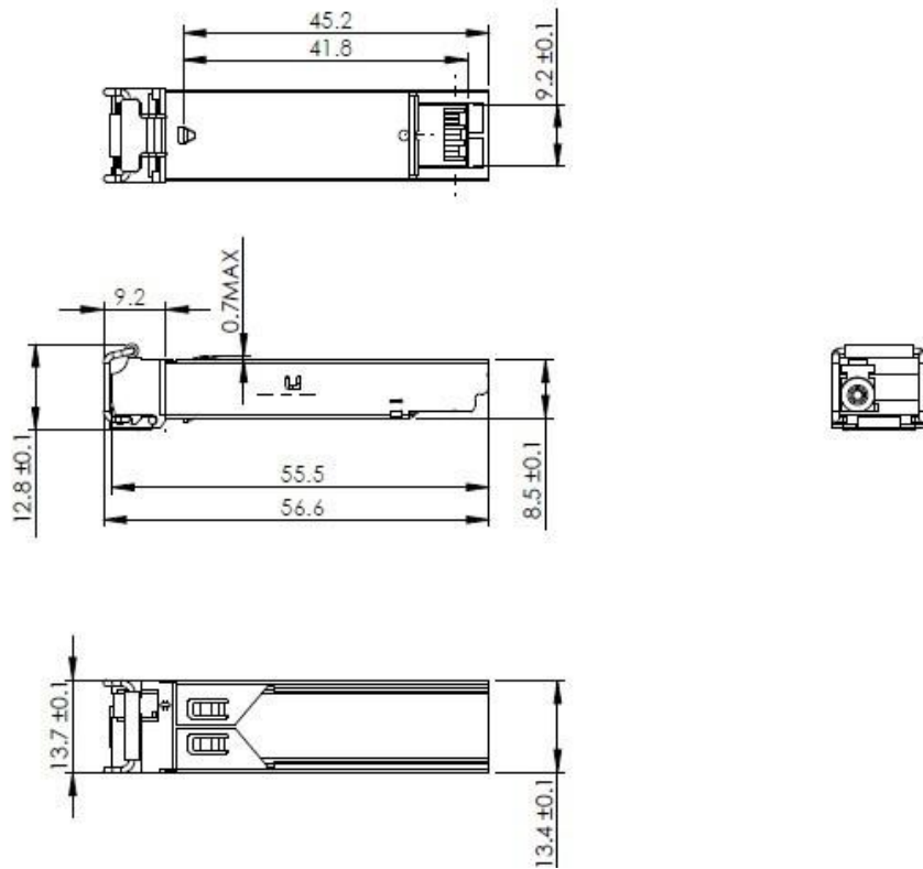
Mechanical Drawing
