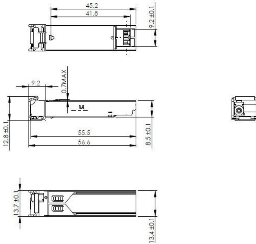
Mechanical Drawing
