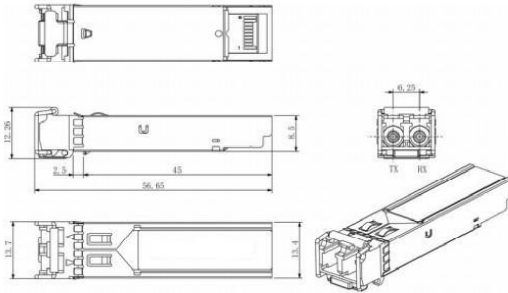
Mechanical Drawing
